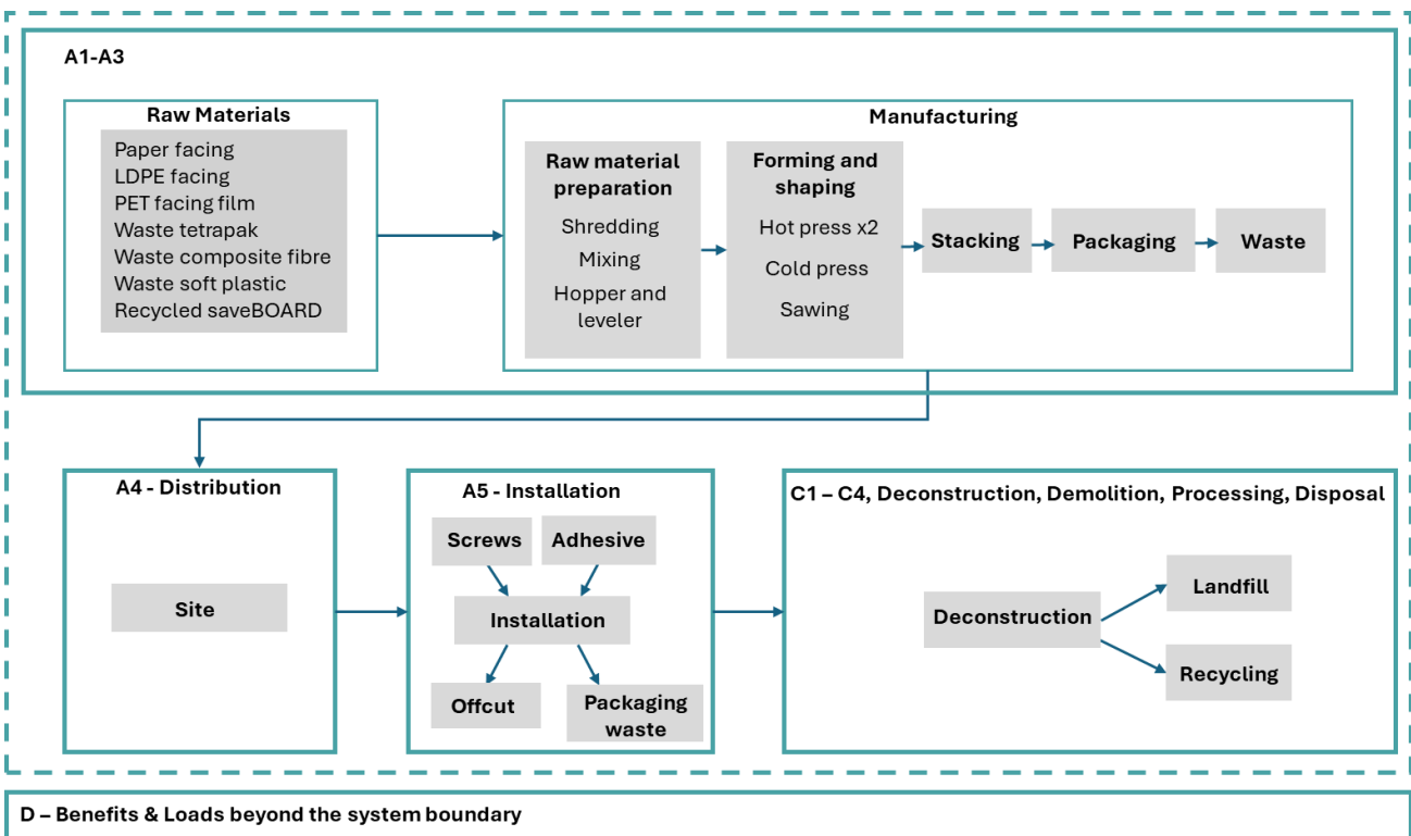
Figure 1 System Diagram
